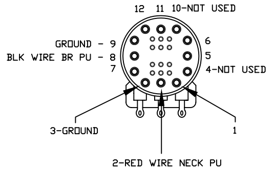
S-1 SWITCH WIRING DETAIL
